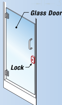
Lock on Single Door Glass-to-Wall
