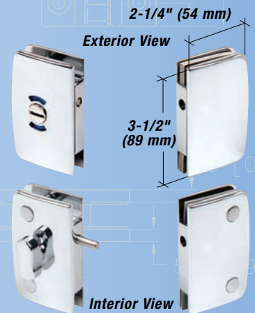
Product Code L-LSW Lock
